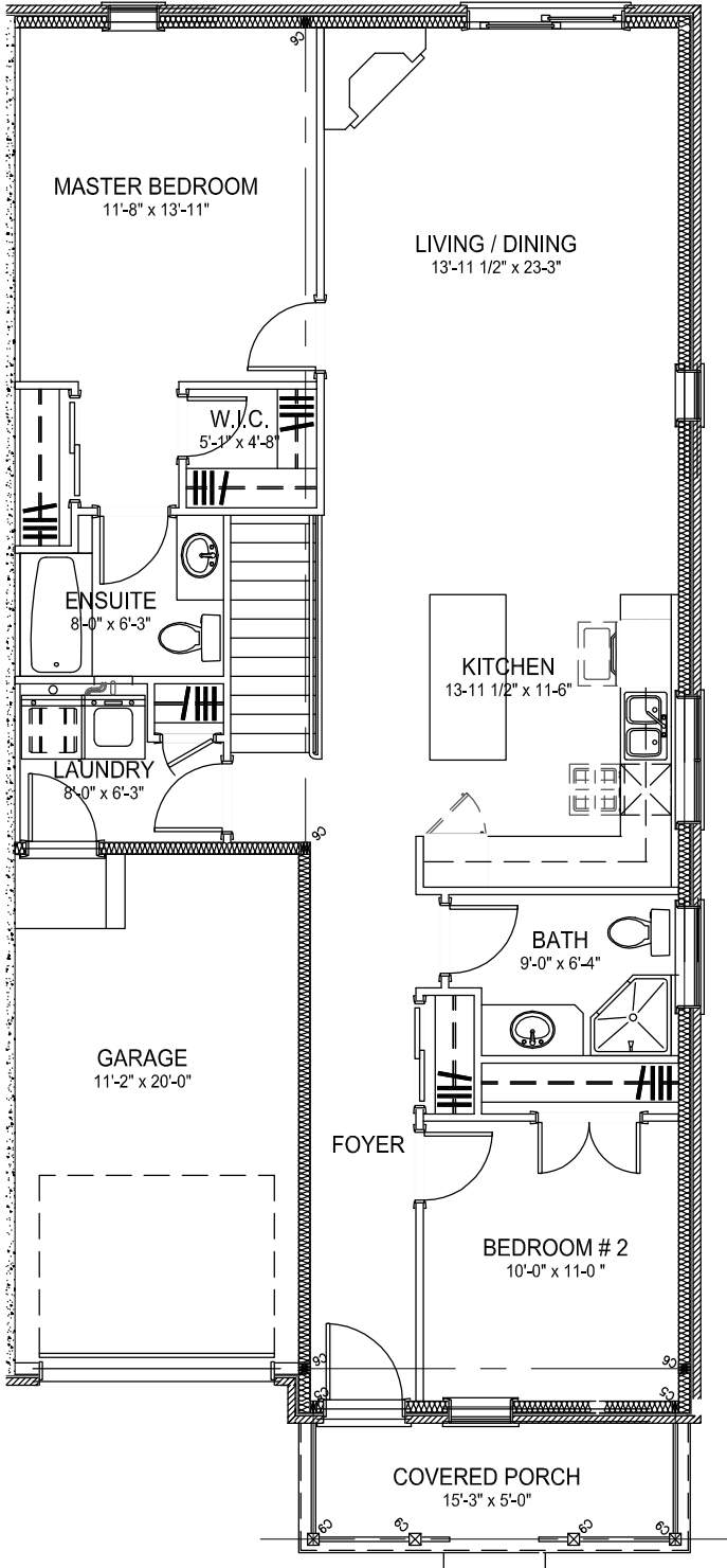
End Unit Floorplan
